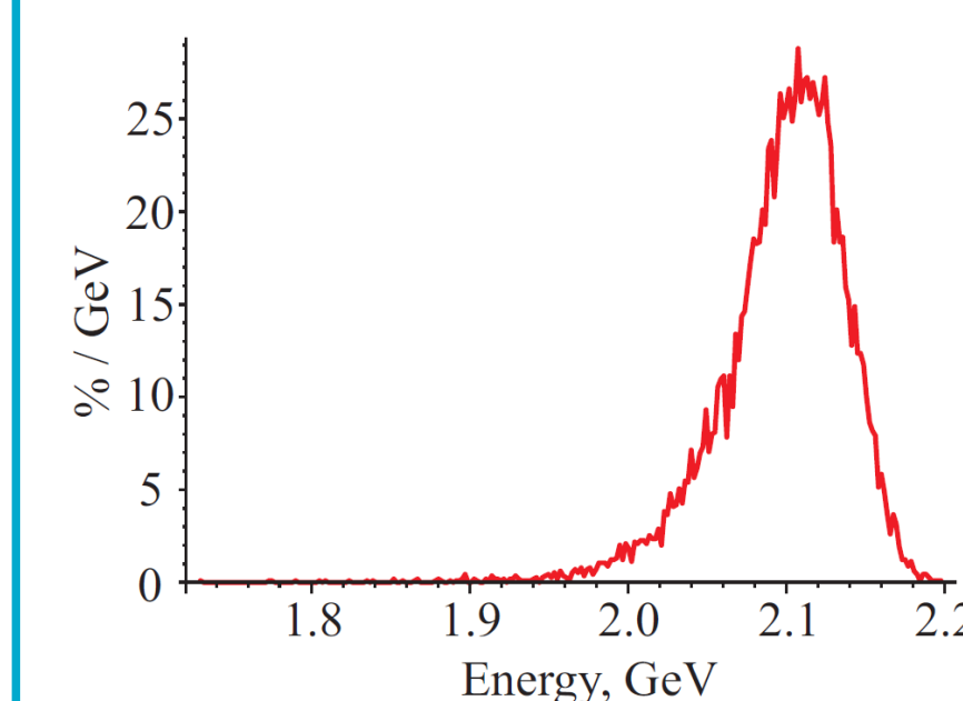
Figure 5: Histogram of the energy spectrum of the captured and accelerated electron beam. A 16 MeV electron beam is injected into a uniform plasma at 4 m, accelerated to over 2 GeV over 6 m, exhibiting a narrow energy spread.
