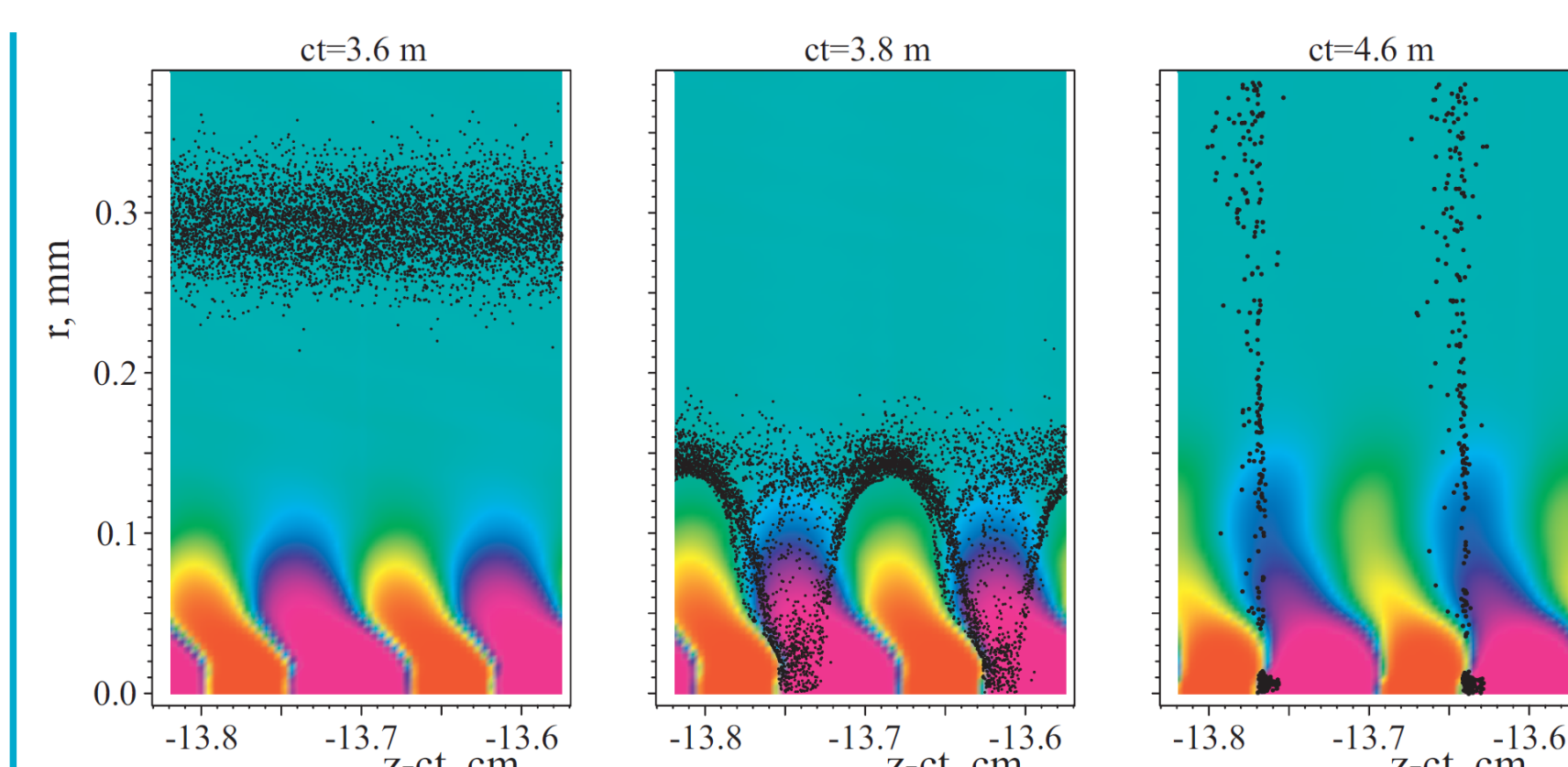
Figure 4: Example of the electron capture process. A long & narrow bunch of electrons (in black) are injected at a shallow angle (5-20 mrad) to the proton beam axis, into the potential wells of the plasma wakefield. The beams are designed to intersect after 4 m of propagation, but electrons are "pulled-in" earlier. After a metre of co-propagation, the majority of electrons are focused into a train of micro-bunches.
