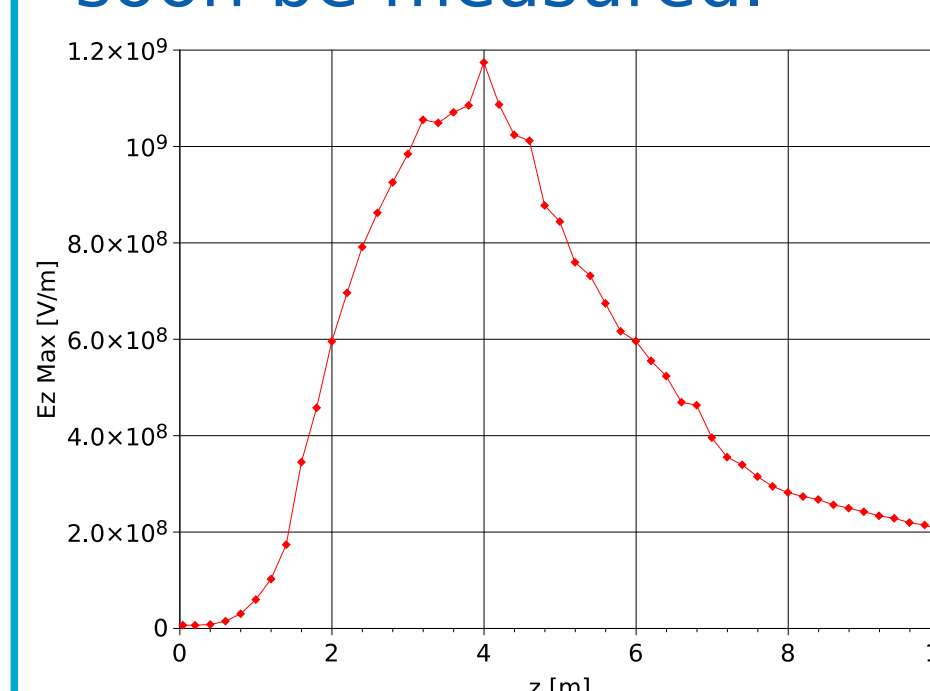
Figure 6: Independent simulation of the AWAKE experiment maximum longitudinal electric field versus beam propagation distance. The simulation was performed using a custom code environment utilising LCODE at its core.
