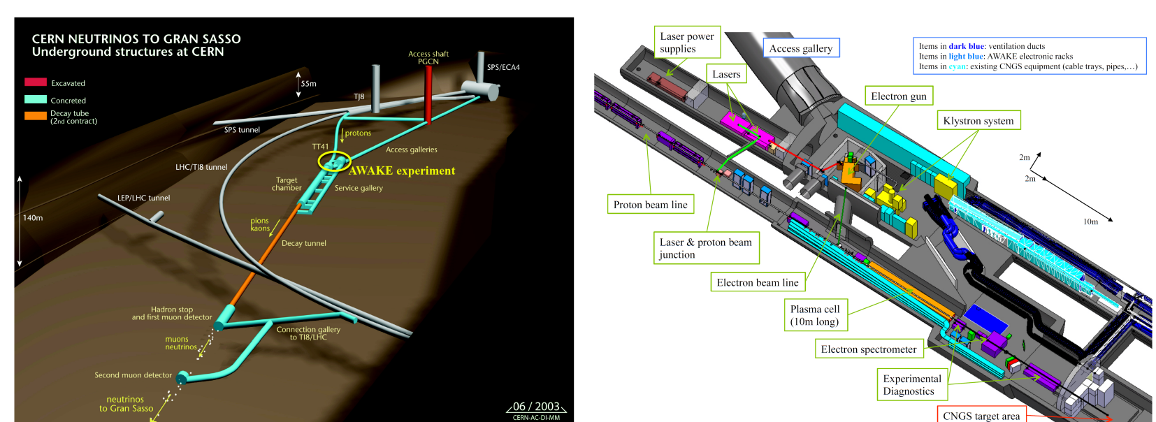
Figure 2: Proposed location of the AWAKE experiment at CERN, and experimental layout. The SPS proton beam is injected into the plasma cell. A terawatt class laser is fired simultaneously to ionise the plasma. The protons drive the wakefield deep into the plasma where the electrons are side-injected, captured and accelerated by the wakefield.
