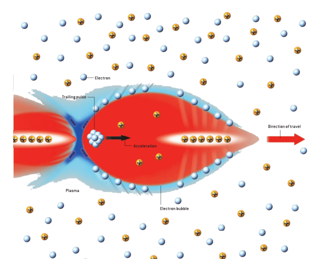
Figure 1: From [1]: Electrons are shifted from their equilibrium positions by Coulomb interactions with the proton beam, whilst ions remain in place. Huge forces now exist between the ions & electrons perpendicular to the beam, causing the electrons to oscillate transversely. This is a plasma wakefield.
