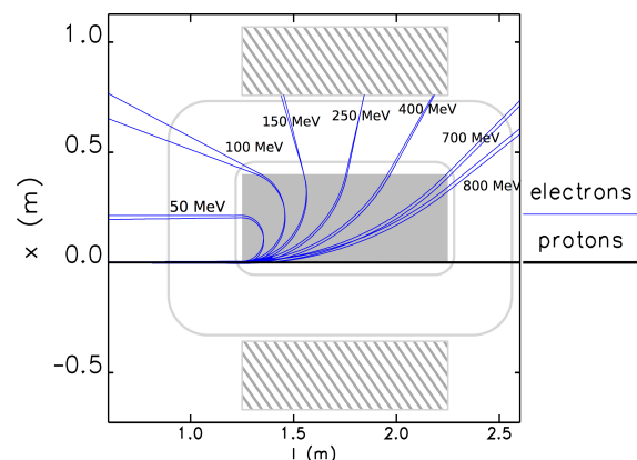
Figure 2: Electron trajectories within the spectrometer dipole for a range of energies.
