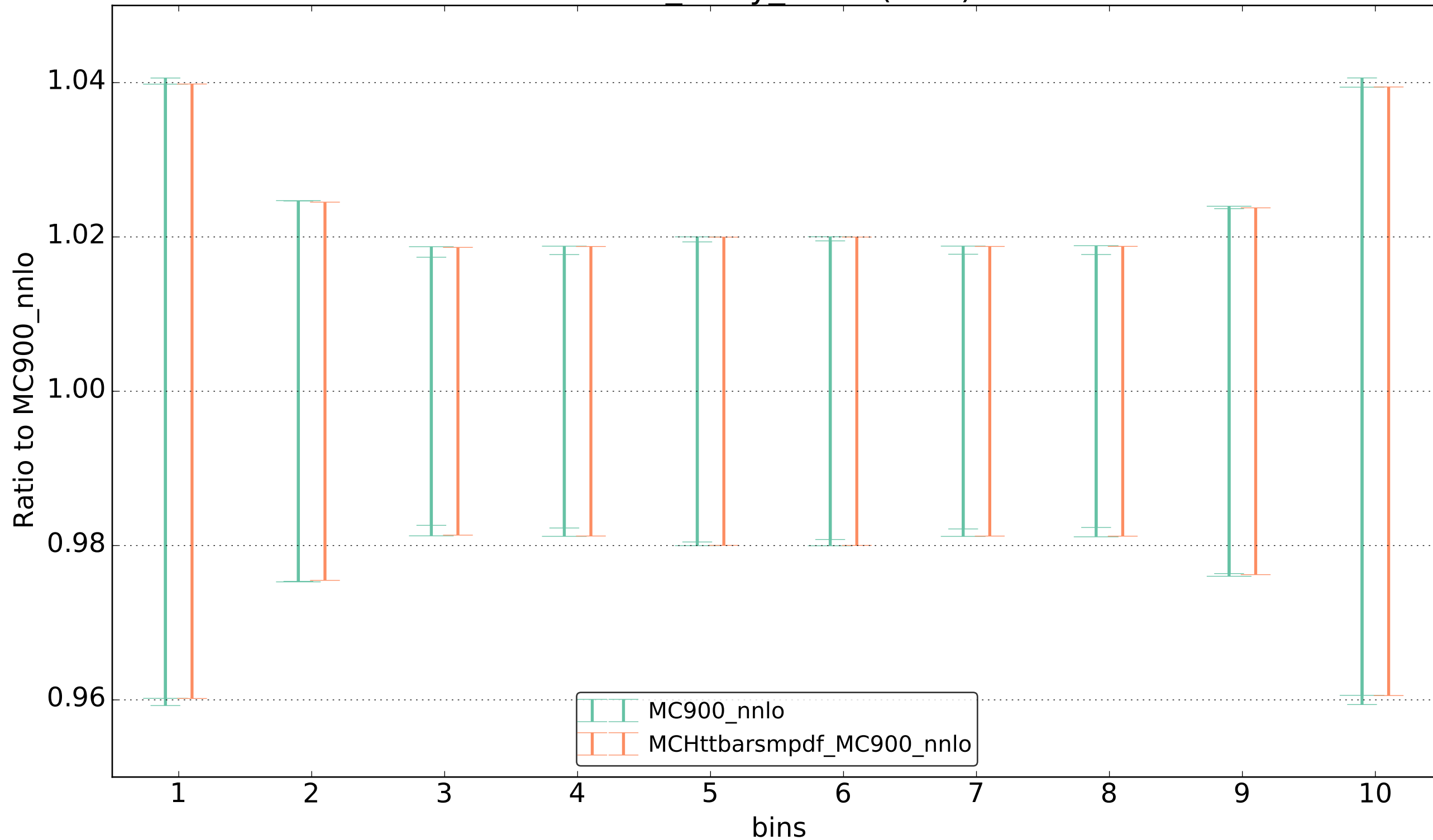
ttbar tbary_13tev(NLO)
