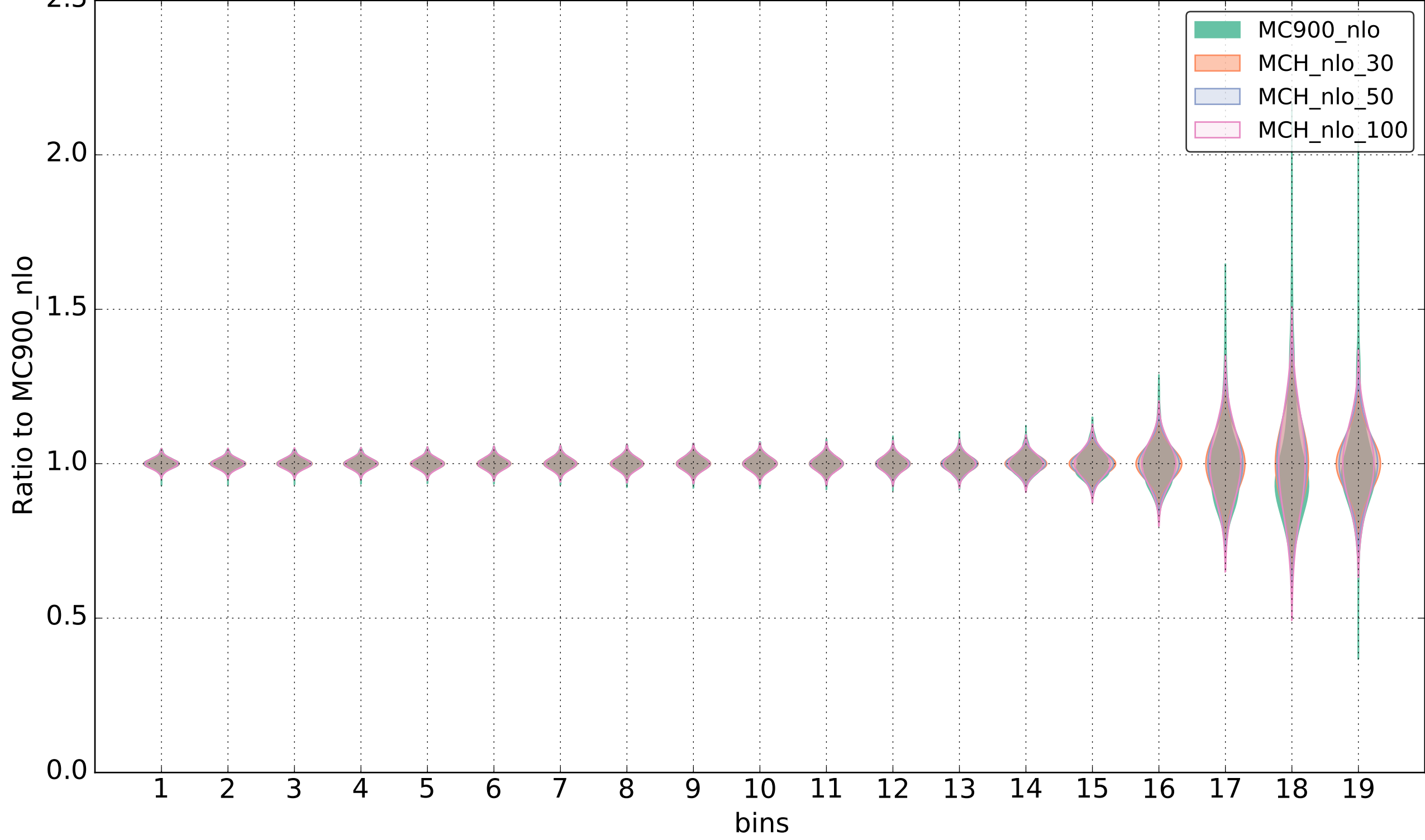
APPLgrid-LHCb-Z0-mumu-eta34(NLO)
