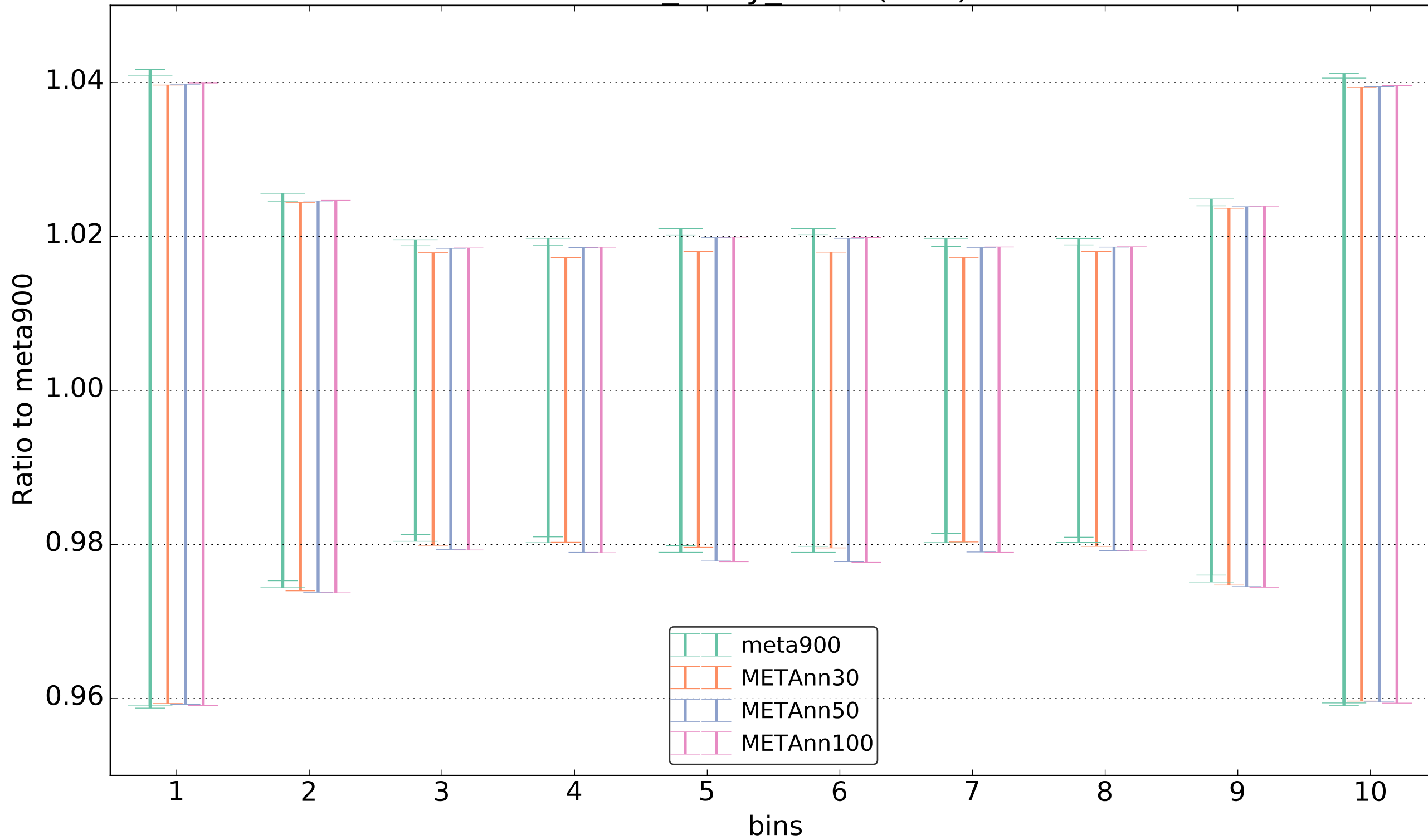
ttbar tbary_13tev(NLO)
